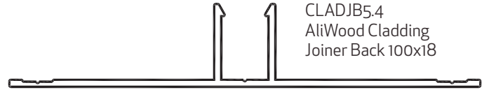
CLADJF5.4 AliWood Cladding Joiner Front 50x15
