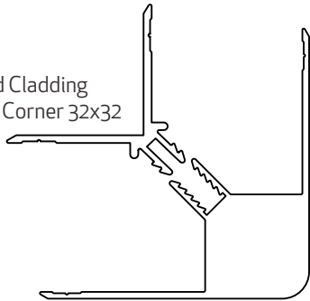
CCLADEC AliWood Castellated Cladding External Corner 60x60
